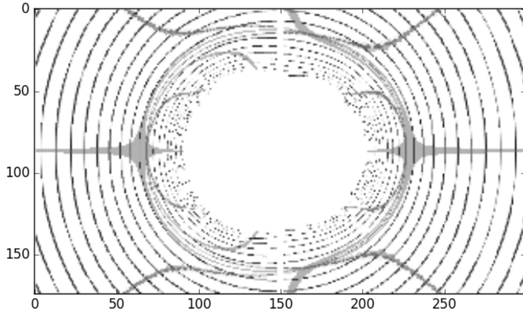
Frutos (m=0.3, a=0.1, e=0.1, q=-0.1)
