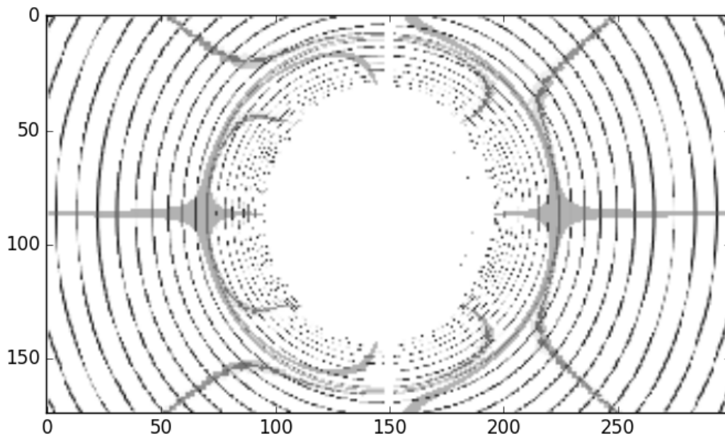
Kerr-Newman (m=0.3, a=0.1, e=1)
