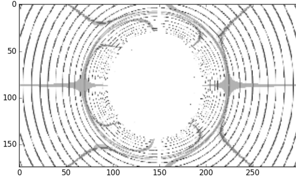
Kerr (m=0.3, a=0.1)
